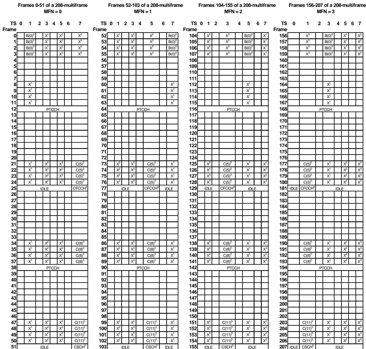
Figure D.7: Example of COMPACT downlink timeslot mapping and rotation of control channels using 4 time groups for nominal cells (based on an assignment of 1 CPBCCCH and 3 CPCCCHs with NIB_CPBCCH_0 = NIB_CPBCCH_1 = NIB_CPBCCH_2 = NIB_CPBCCH_3 = 1 and NIB_CPCCCH_0 = NIB_CPCCCH_2 = NIB_CPCCCH_3 = 3, NIB_CPCCCH_1 = 4). TG = 0 is illustrated. NIB_CPBCCH and NIB_CPCCCH are not broadcast for serving cell time group.
