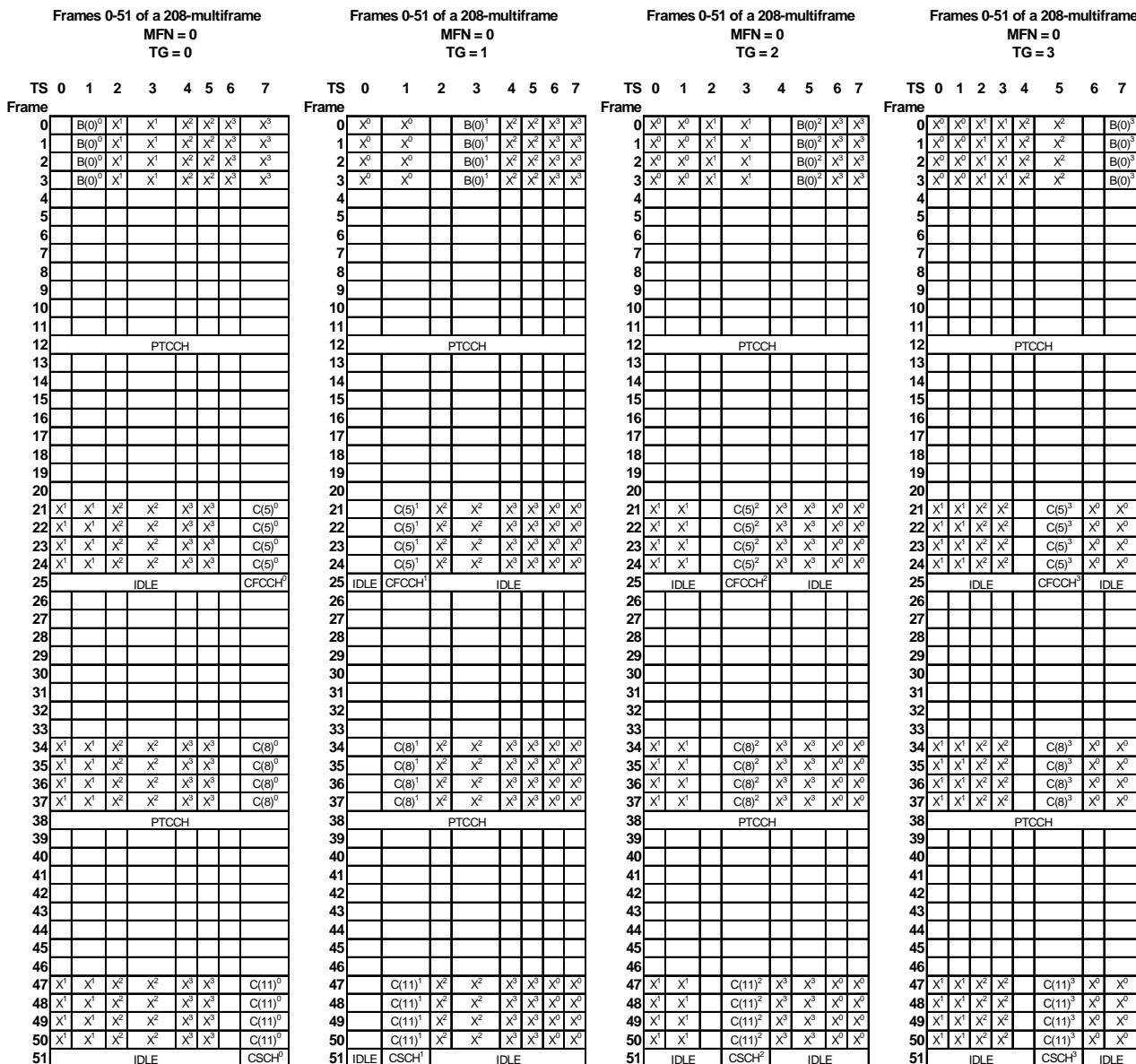
Figure D.3: COMPACT downlink 52-multiframe structure using 4 time groups for large cells (based on an assignment of 1 CPBCCCH and 3 CPCCCHs with NIB_CPBCCCH_0 = NIB_CPBCCCH_1 = NIB_CPBCCCH_2 = NIB_CPBCCCH_3 = 1 and NIB_CPCCCH_0 = NIB_CPCCCH_1 = NIB_CPCCCH_2 = NIB_CPCCCH_3 = 3). NIB_CPBCCCH and NIB_CPCCCH are not broadcast for serving cell time group.
