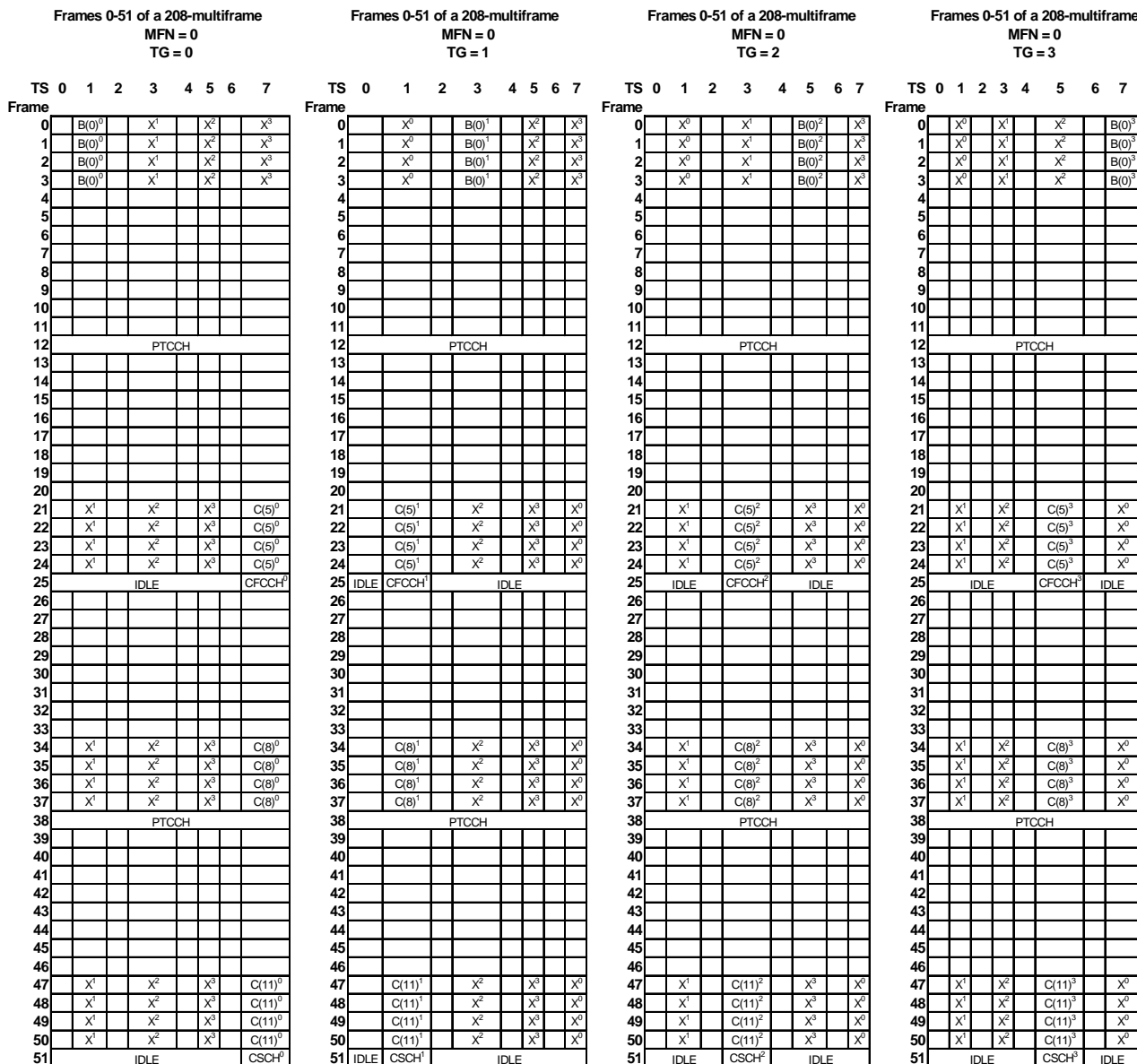
Figure D.1: COMPACT downlink 52-multiframe structure using 4 time groups for nominal cells (based on an assignment of 1 CPBCCCH and 3 CPCCCHs with NIB_CPBCCCH_0 = NIB_CPBCCCH_1 = NIB_CPBCCCH_2 = NIB_CPBCCCH_3 = 1 and NIB_CPCCCH_0 = NIB_CPCCCH_1 = NIB_CPCCCH_2 = NIB_CPCCCH_3 = 3). NIB_CPBCCCH and NIB_CPCCCH are not broadcast for serving cell time group.
