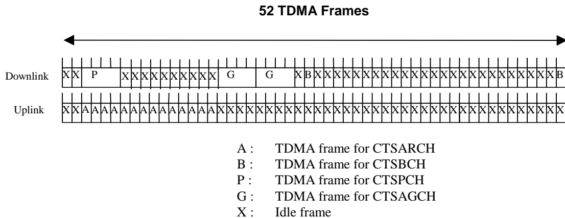
Figure 10: 52-multiframe for CTS
